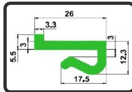
COLLAR TYPE 26MM
