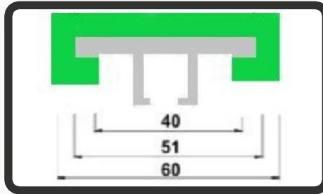
C TYPE 60X51 + ALU PROFILE
