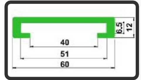
C TYPE 60X51
