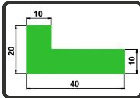
L TYPE 40X20X10
