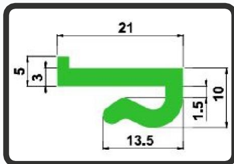
COLLAR TYPE 21MM
