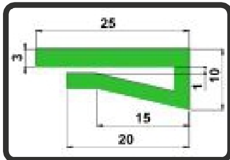
CLIP TYPE 25MM
