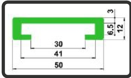
C TYPE 50X41
